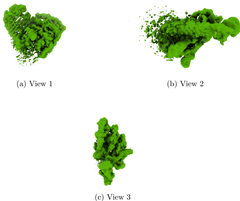
Figure 4: Isosurface at threshold=0.004950. Views generated by ChimeraX at a the following X, Y, Z angles: View 1 (0, -90, -90), View 2 (-90, 0, -90), View 3 (0, 0, 0).
