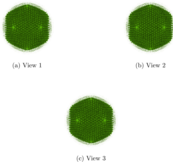
Figure 4: Isosurface at threshold=2.010000. Views generated by ChimeraX at a the following X, Y, Z angles: View 1 (0, -90, -90), View 2 (-90, 0, -90), View 3 (0, 0, 0).
