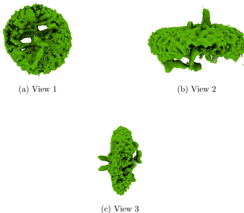
Figure 4: Isosurface at threshold=0.006400. Views generated by ChimeraX at a the following X, Y, Z angles: View 1 (0, -90, -90), View 2 (-90, 0, -90), View 3 (0, 0, 0).
