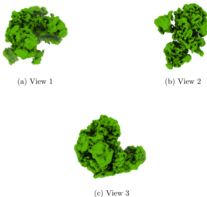
Figure 4: Isosurface at threshold=0.128000. Views generated by ChimeraX at a the following X, Y, Z angles: View 1 (0, -90, -90), View 2 (-90, 0, -90), View 3 (0, 0, 0).
