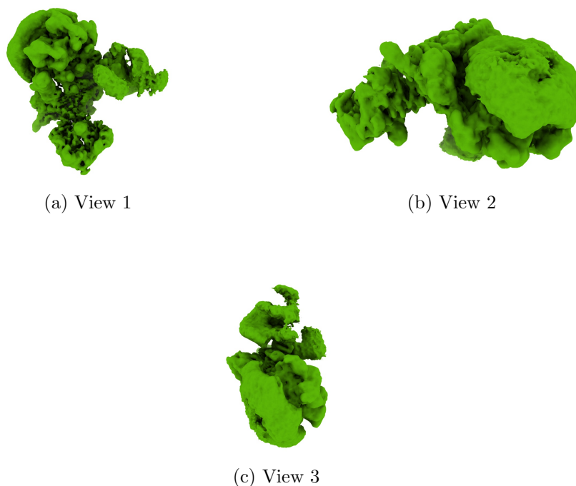
Figure 4: Isosurface at threshold=0.552000. Views generated by ChimeraX at a the following X, Y, Z angles: View 1 (0, -90, -90), View 2 (-90, 0, -90), View 3 (0, 0, 0).
