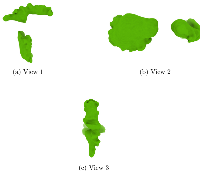
Figure 4: Isosurface at threshold=0.027000. Views generated by ChimeraX at a the following X, Y, Z angles: View 1 (0, -90, -90), View 2 (-90, 0, -90), View 3 (0, 0, 0).
