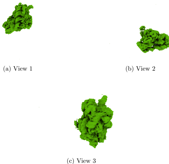
Figure 4: Isosurface at threshold=0.578000. Views generated by ChimeraX at a the following X, Y, Z angles: View 1 (0, -90, -90), View 2 (-90, 0, -90), View 3 (0, 0, 0).
