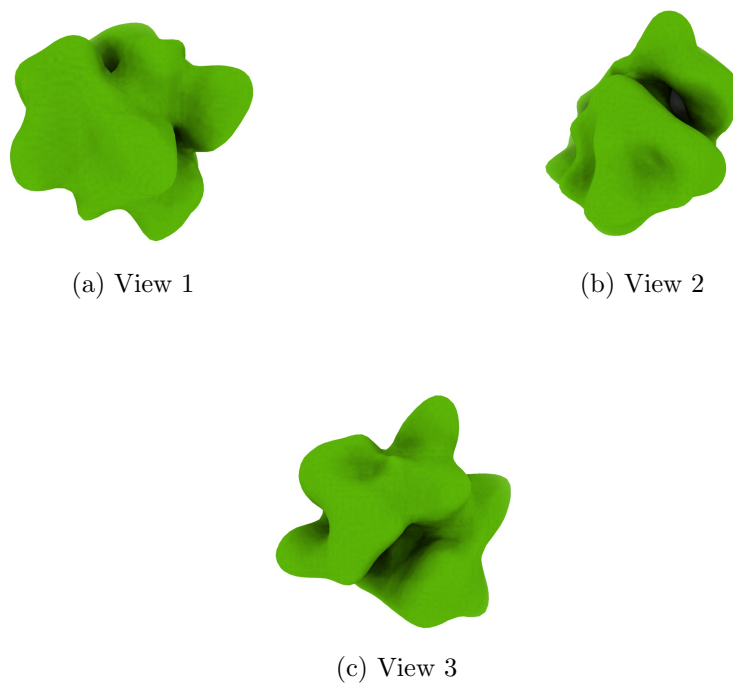
Figure 4: Isosurface at threshold=150.000000. Views generated by ChimeraX at a the following X, Y, Z angles: View 1 (0, -90, -90), View 2 (-90, 0, -90), View 3 (0, 0, 0).
