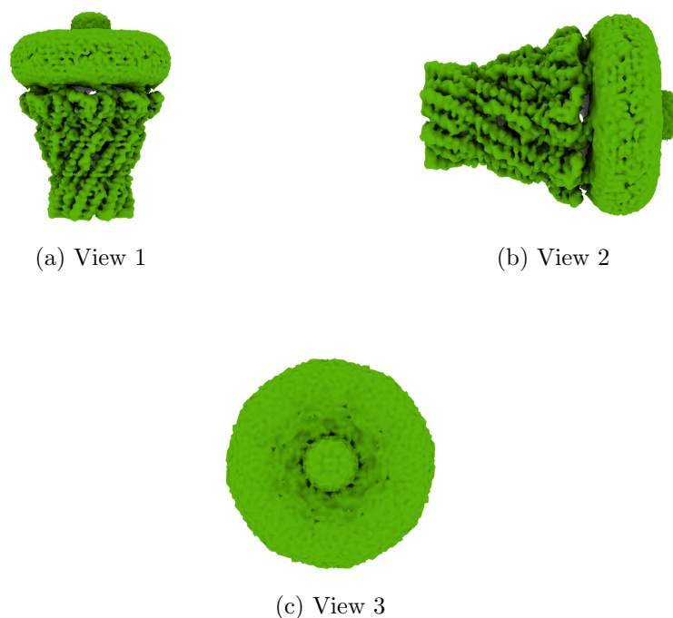
Figure 4: Isosurface at threshold=0.110000. Views generated by ChimeraX at the following X, Y, Z angles: View 1 (0, -90, -90), View 2 (-90, 0, -90), View 3 (0, 0, 0).
