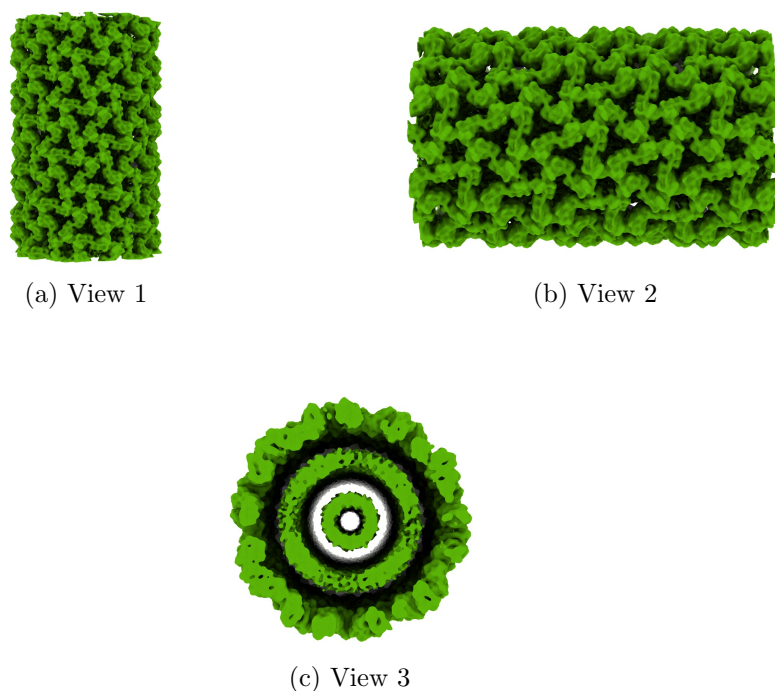
Figure 4: Isosurface at threshold=4.000000. Views generated by ChimeraX at the following X, Y, Z angles: View 1 (0, -90, -90), View 2 (-90, 0, -90), View 3 (0, 0, 0).
