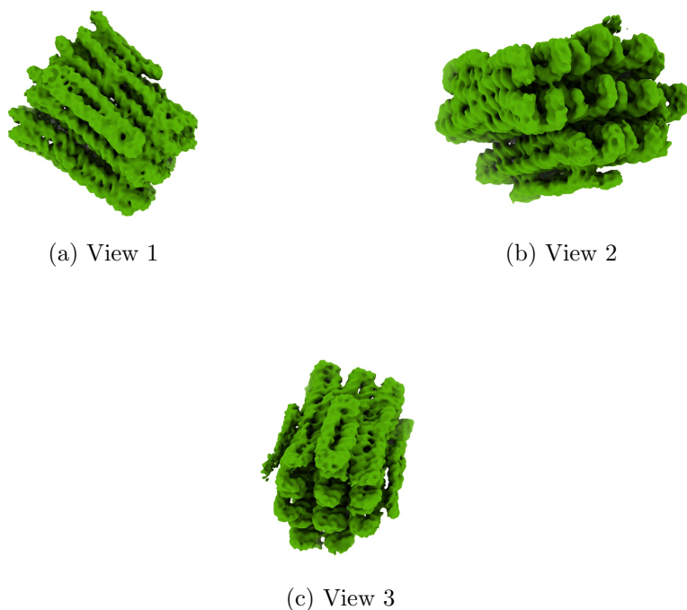
Figure 4: Isosurface at threshold=0.040400. Views generated by ChimeraX at a the following X, Y, Z angles: View 1 (0, -90, -90), View 2 (-90, 0, -90), View 3 (0, 0, 0).
