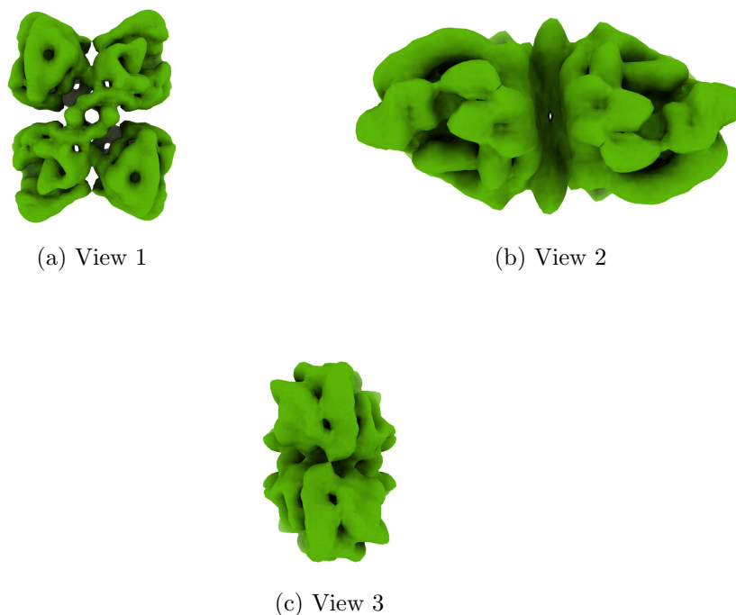
Figure 4: Isosurface at threshold=0.027000. Views generated by ChimeraX at a the following X, Y, Z angles: View 1 (0, -90, -90), View 2 (-90, 0, -90), View 3 (0, 0, 0).
