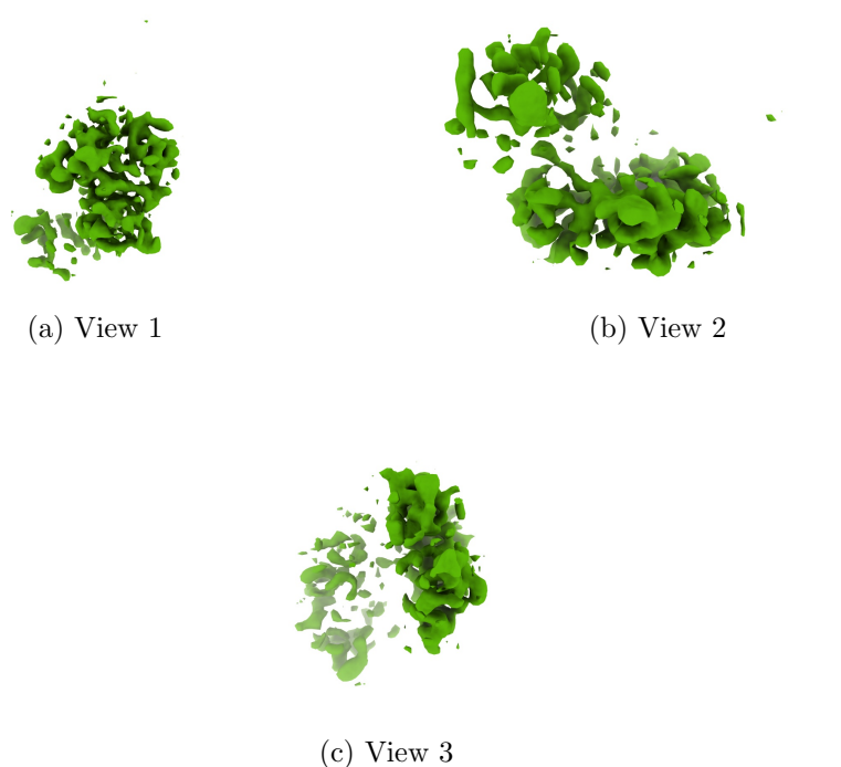
Figure 4: Isosurface at threshold=4.560000. Views generated by ChimeraX at a the following X, Y, Z angles: View 1 (0, -90, -90), View 2 (-90, 0, -90), View 3 (0, 0, 0).
