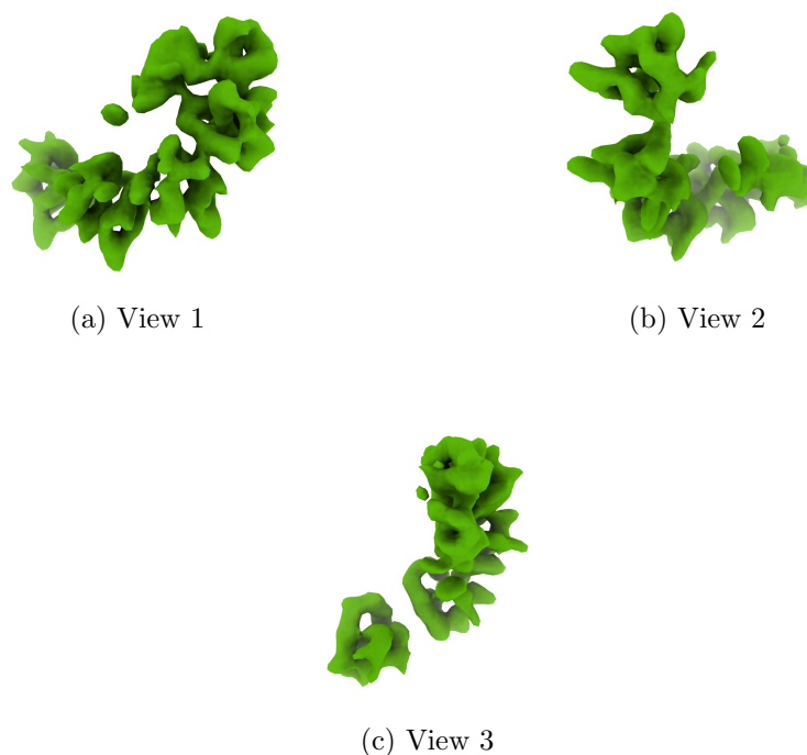
Figure 4: Isosurface at threshold=0.210000. Views generated by ChimeraX at a the following X, Y, Z angles: View 1 (0, -90, -90), View 2 (-90, 0, -90), View 3 (0, 0, 0).
