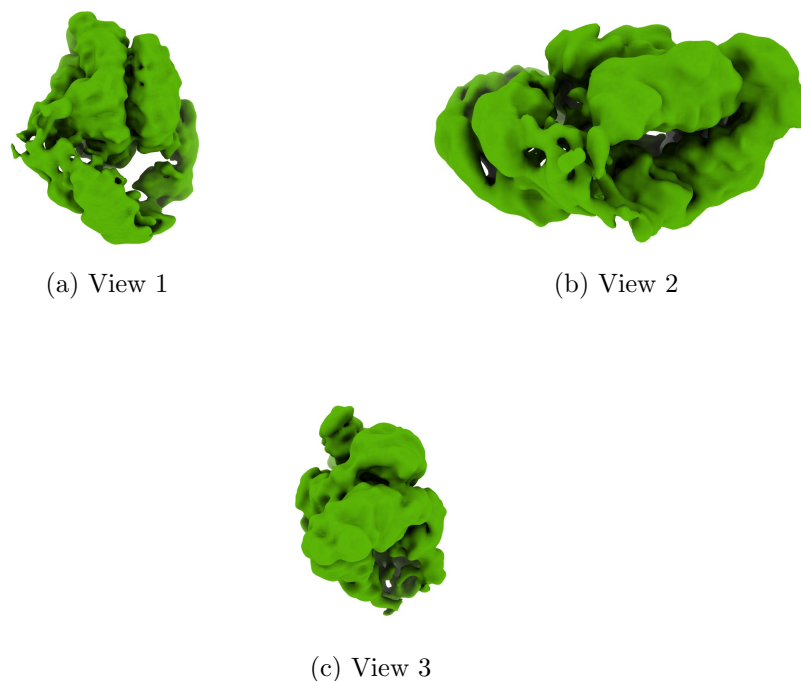
Figure 4: Isosurface at threshold=1.040000. Views generated by ChimeraX at a the following X, Y, Z angles: View 1 (0, -90, -90), View 2 (-90, 0, -90), View 3 (0, 0, 0).
