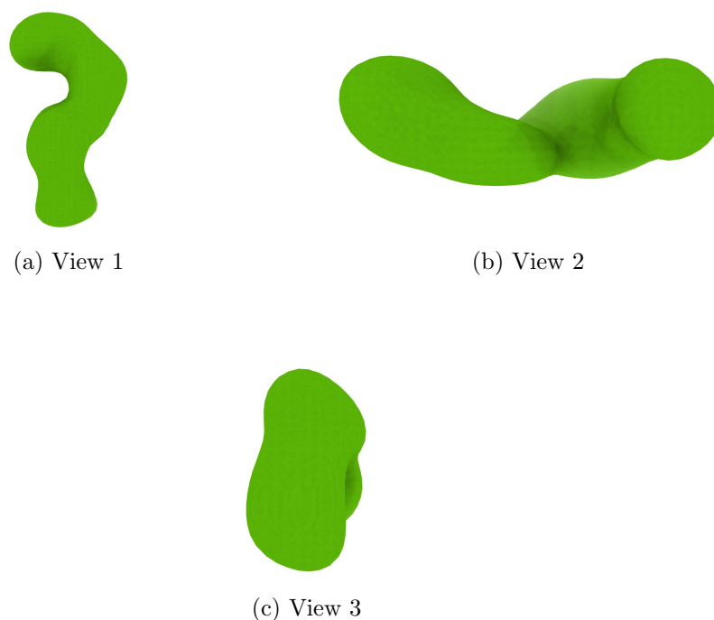
Figure 4: Isosurface at threshold=2.900000. Views generated by ChimeraX at a the following X, Y, Z angles: View 1 (0, -90, -90), View 2 (-90, 0, -90), View 3 (0, 0, 0).
