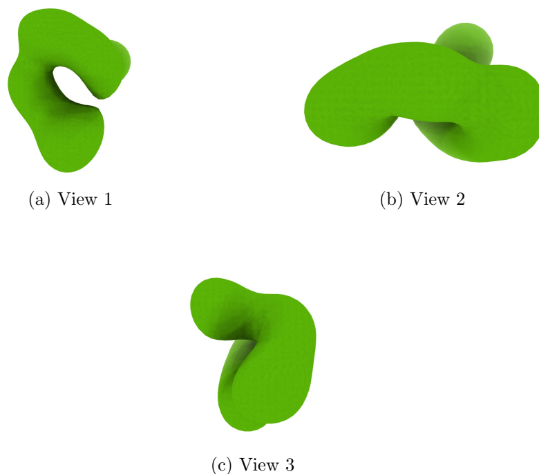
Figure 4: Isosurface at threshold=2.760000. Views generated by ChimeraX at a the following X, Y, Z angles: View 1 (0, -90, -90), View 2 (-90, 0, -90), View 3 (0, 0, 0).
