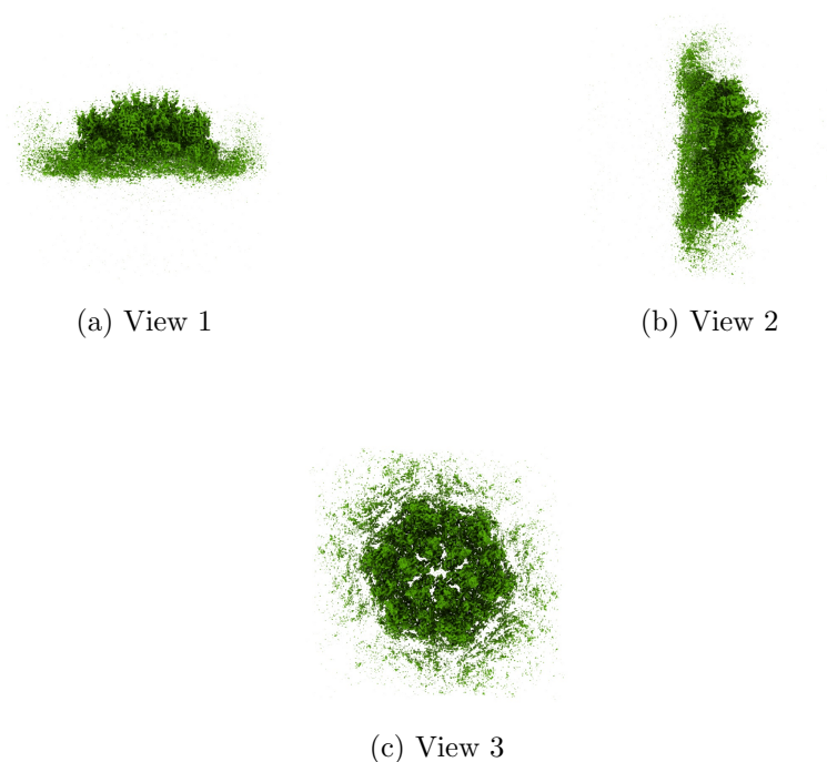
Figure 4: Isosurface at threshold=0.008700. Views generated by ChimeraX at a the following X, Y, Z angles: View 1 (0, -90, -90), View 2 (-90, 0, -90), View 3 (0, 0, 0).
