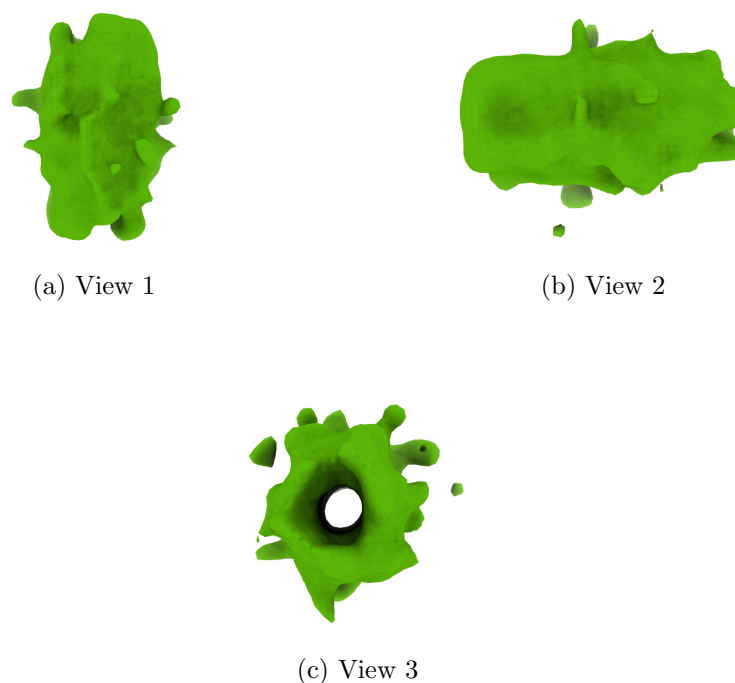
Figure 4: Isosurface at threshold=0.054000. Views generated by ChimeraX at a the following X, Y, Z angles: View 1 (0, -90, -90), View 2 (-90, 0, -90), View 3 (0, 0, 0).
