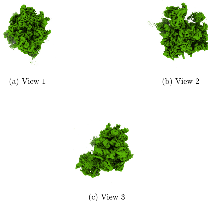
Figure 4: Isosurface at threshold=2.200000. Views generated by ChimeraX at a the following X, Y, Z angles: View 1 (0, -90, -90), View 2 (-90, 0, -90), View 3 (0, 0, 0).
