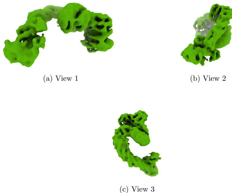
Figure 4: Isosurface at threshold=0.030000. Views generated by ChimeraX at a the following X, Y, Z angles: View 1 (0, -90, -90), View 2 (-90, 0, -90), View 3 (0, 0, 0).
