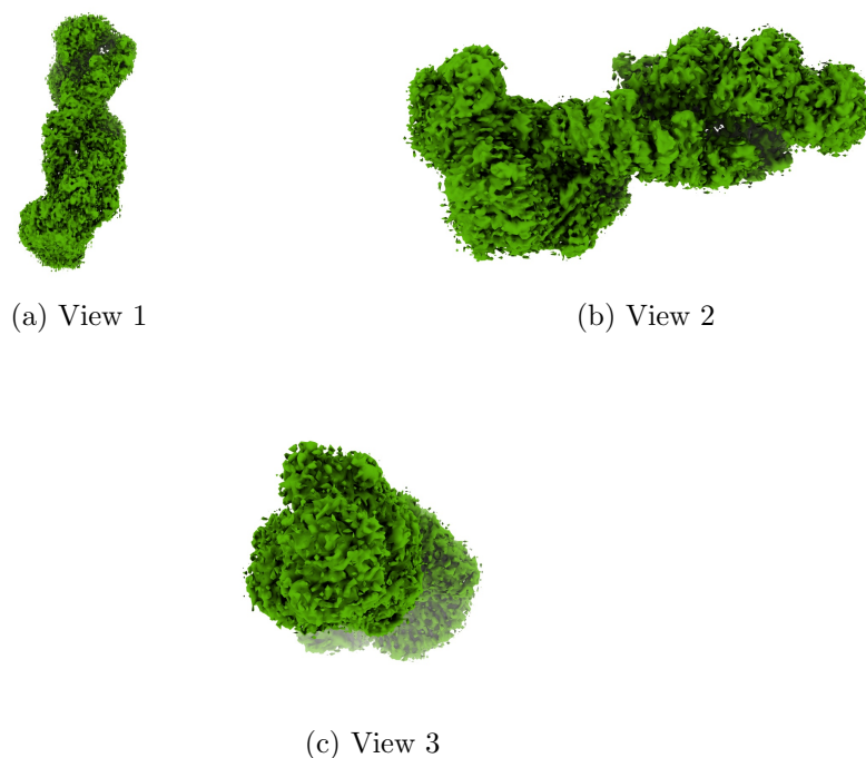
Figure 4: Isosurface at threshold=0.007000. Views generated by ChimeraX at a the following X, Y, Z angles: View 1 (0, -90, -90), View 2 (-90, 0, -90), View 3 (0, 0, 0).
