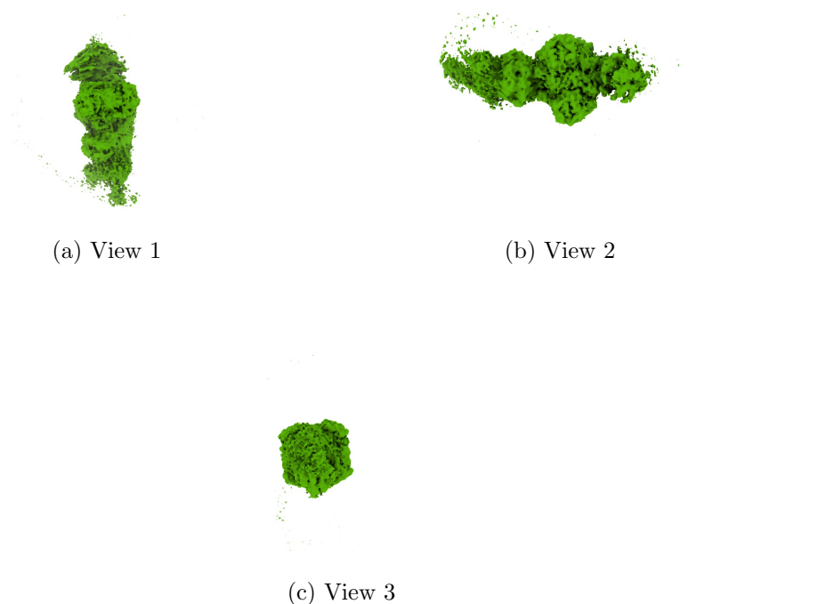
Figure 4: Isosurface at threshold=0.003000. Views generated by ChimeraX at a the following X, Y, Z angles: View 1 (0, -90, -90), View 2 (-90, 0, -90), View 3 (0, 0, 0).
