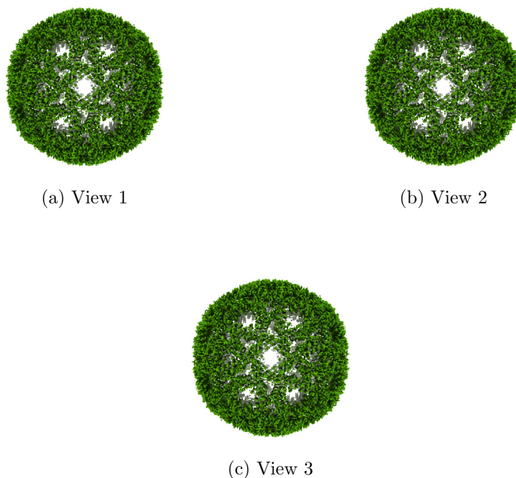
Figure 4: Isosurface at threshold=0.034700. Views generated by ChimeraX at a the following X, Y, Z angles: View 1 (0, -90, -90), View 2 (-90, 0, -90), View 3 (0, 0, 0).
