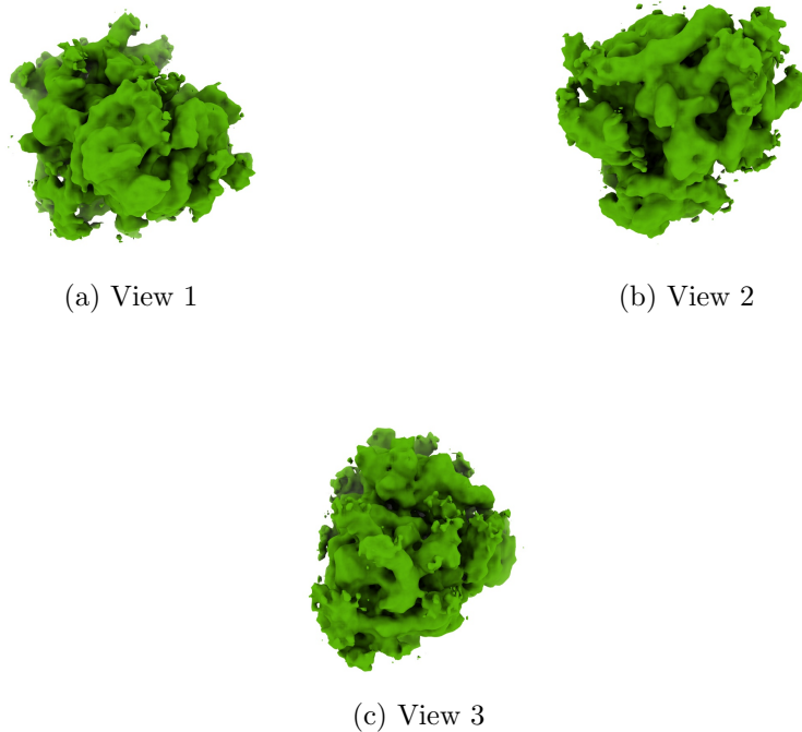
Figure 4: Isosurface at threshold=0.001180. Views generated by ChimeraX at a the following X, Y, Z angles: View 1 (0, -90, -90), View 2 (-90, 0, -90), View 3 (0, 0, 0).
