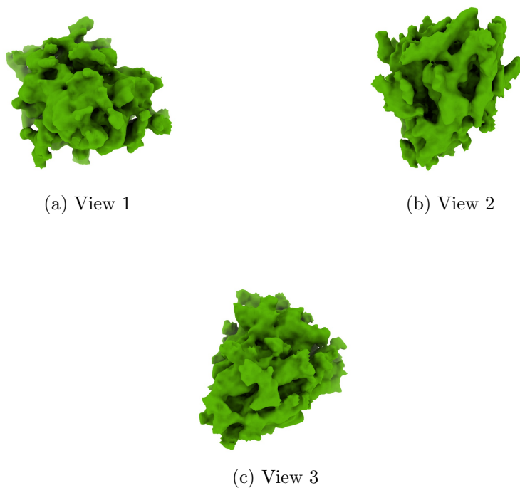
Figure 4: Isosurface at threshold=18.000000. Views generated by ChimeraX at a the following X, Y, Z angles: View 1 (0, -90, -90), View 2 (-90, 0, -90), View 3 (0, 0, 0).
