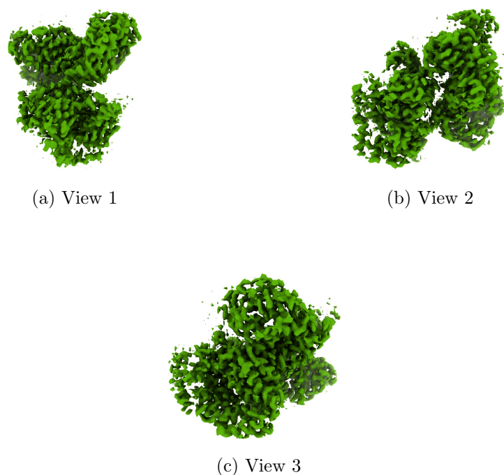
Figure 4: Isosurface at threshold=0.004500. Views generated by ChimeraX at a the following X, Y, Z angles: View 1 (0, -90, -90), View 2 (-90, 0, -90), View 3 (0, 0, 0).
