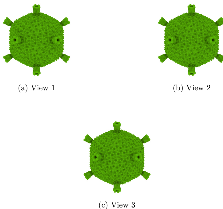
Figure 4: Isosurface at threshold=960.000000. Views generated by ChimeraX at a the following X, Y, Z angles: View 1 (0, -90, -90), View 2 (-90, 0, -90), View 3 (0, 0, 0).
