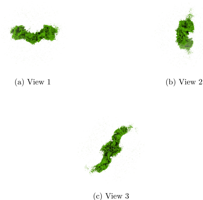
Figure 4: Isosurface at threshold=0.056000. Views generated by ChimeraX at a the following X, Y, Z angles: View 1 (0, -90, -90), View 2 (-90, 0, -90), View 3 (0, 0, 0).
