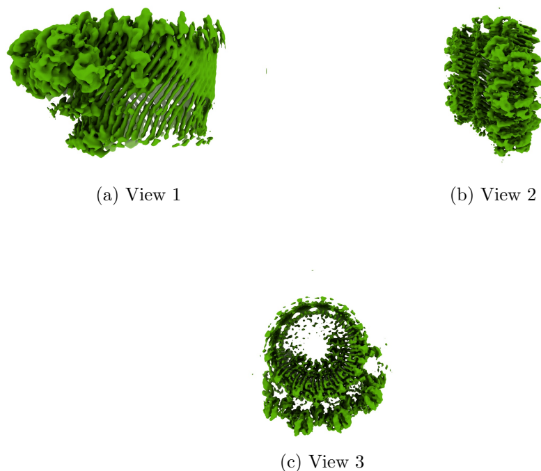
Figure 4: Isosurface at threshold=0.013000. Views generated by ChimeraX at a the following X, Y, Z angles: View 1 (0, -90, -90), View 2 (-90, 0, -90), View 3 (0, 0, 0).
