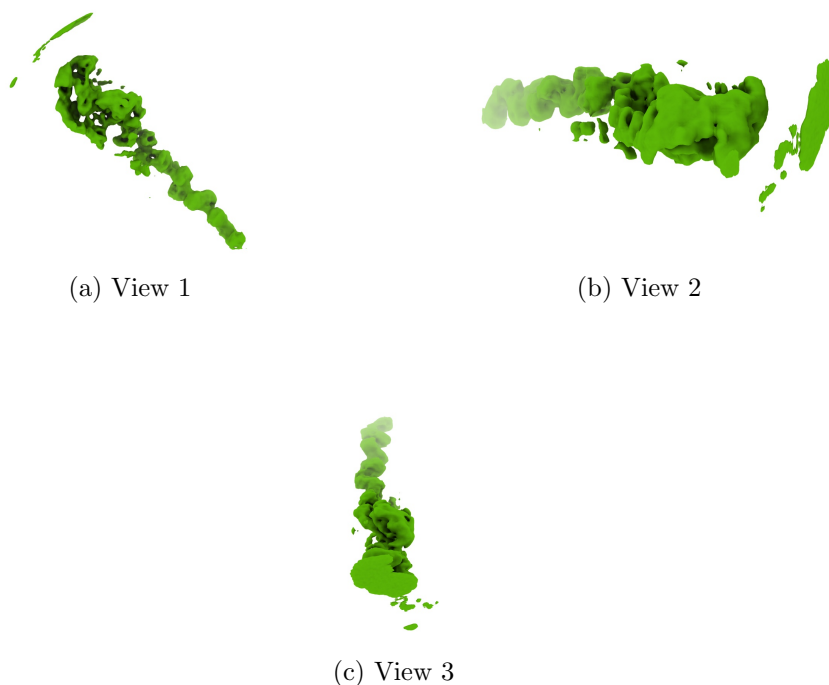
Figure 4: Isosurface at threshold=0.280000. Views generated by ChimeraX at a the following X, Y, Z angles: View 1 (0, -90, -90), View 2 (-90, 0, -90), View 3 (0, 0, 0).
