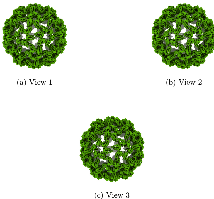
Figure 4: Isosurface at threshold=0.189000. Views generated by ChimeraX at a the following X, Y, Z angles: View 1 (0, -90, -90), View 2 (-90, 0, -90), View 3 (0, 0, 0).
