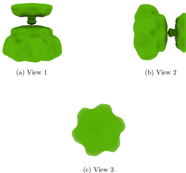
Figure 4: Isosurface at threshold=1.670000. Views generated by ChimeraX at a the following X, Y, Z angles: View 1 (0, -90, -90), View 2 (-90, 0, -90), View 3 (0, 0, 0).
