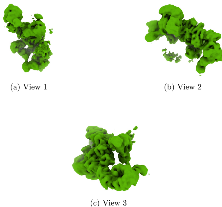
Figure 4: Isosurface at threshold=0.027300. Views generated by ChimeraX at a the following X, Y, Z angles: View 1 (0, -90, -90), View 2 (-90, 0, -90), View 3 (0, 0, 0).
