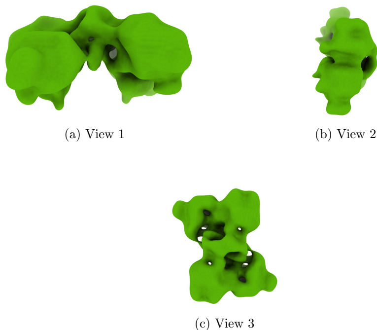
Figure 4: Isosurface at threshold=0.057300. Views generated by ChimeraX at a the following X, Y, Z angles: View 1 (0, -90, -90), View 2 (-90, 0, -90), View 3 (0, 0, 0).
