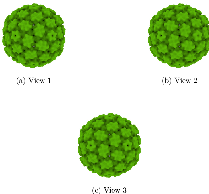
Figure 4: Isosurface at threshold=173.000000. Views generated by ChimeraX at a the following X, Y, Z angles: View 1 (0, -90, -90), View 2 (-90, 0, -90), View 3 (0, 0, 0).
