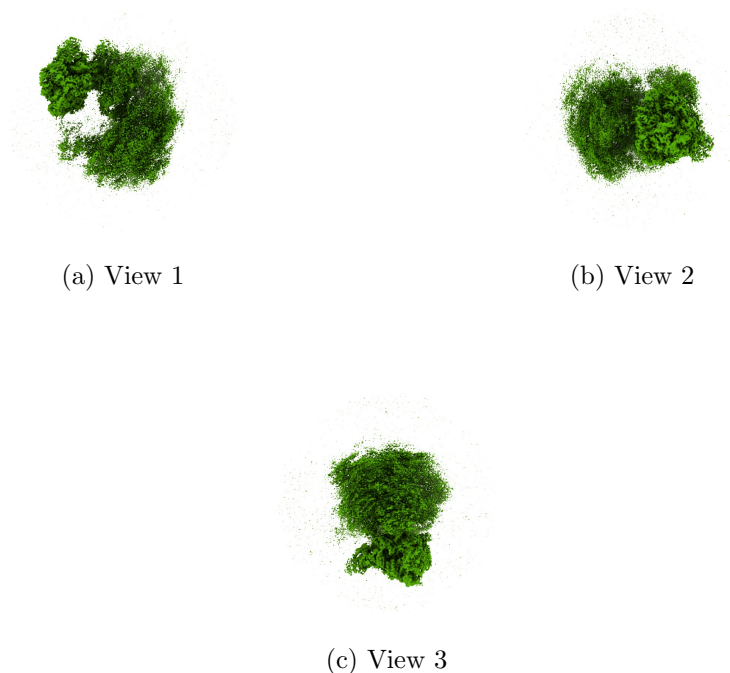
Figure 4: Isosurface at threshold=0.179000. Views generated by ChimeraX at a the following X, Y, Z angles: View 1 (0, -90, -90), View 2 (-90, 0, -90), View 3 (0, 0, 0).
