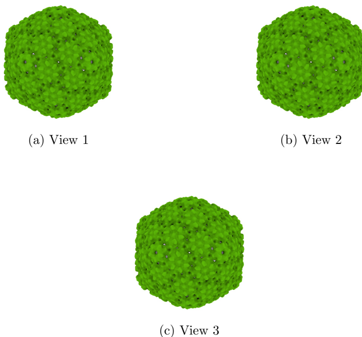
Figure 4: Isosurface at threshold=110.000000. Views generated by ChimeraX at a the following X, Y, Z angles: View 1 (0, -90, -90), View 2 (-90, 0, -90), View 3 (0, 0, 0).
