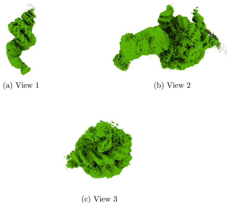
Figure 4: Isosurface at threshold=0.057900. Views generated by ChimeraX at a the following X, Y, Z angles: View 1 (0, -90, -90), View 2 (-90, 0, -90), View 3 (0, 0, 0).
