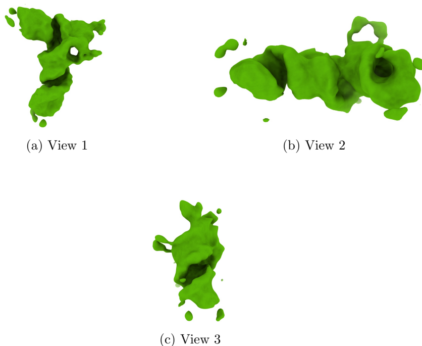
Figure 4: Isosurface at threshold=0.546000. Views generated by ChimeraX at a the following X, Y, Z angles: View 1 (0, -90, -90), View 2 (-90, 0, -90), View 3 (0, 0, 0).
