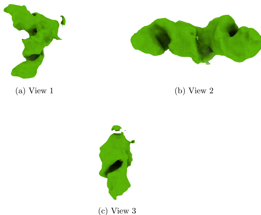
Figure 4: Isosurface at threshold=1.190000. Views generated by ChimeraX at a the following X, Y, Z angles: View 1 (0, -90, -90), View 2 (-90, 0, -90), View 3 (0, 0, 0).
