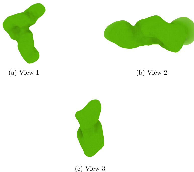
Figure 4: Isosurface at threshold=3.180000. Views generated by ChimeraX at a the following X, Y, Z angles: View 1 (0, -90, -90), View 2 (-90, 0, -90), View 3 (0, 0, 0).
