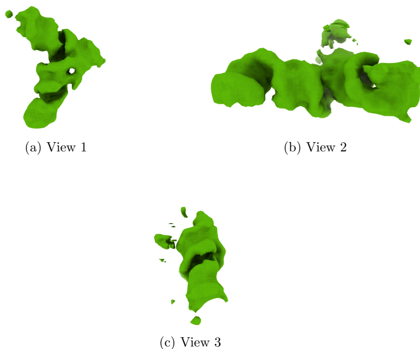
Figure 4: Isosurface at threshold=1.590000. Views generated by ChimeraX at a the following X, Y, Z angles: View 1 (0, -90, -90), View 2 (-90, 0, -90), View 3 (0, 0, 0).
