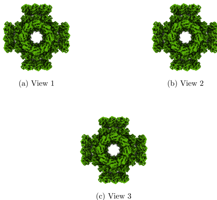
Figure 4: Isosurface at threshold=0.094100. Views generated by ChimeraX at a the following X, Y, Z angles: View 1 (0, -90, -90), View 2 (-90, 0, -90), View 3 (0, 0, 0).
