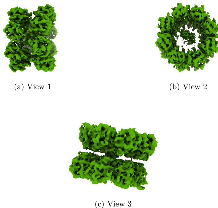
Figure 4: Isosurface at threshold=0.521000. Views generated by ChimeraX at a the following X, Y, Z angles: View 1 (0, -90, -90), View 2 (-90, 0, -90), View 3 (0, 0, 0).
