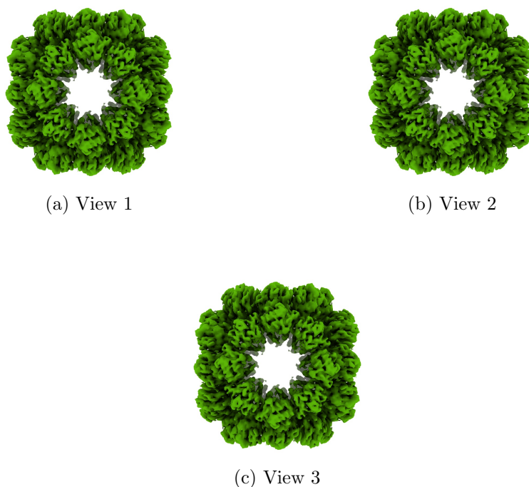
Figure 4: Isosurface at threshold=0.254000. Views generated by ChimeraX at a the following X, Y, Z angles: View 1 (0, -90, -90), View 2 (-90, 0, -90), View 3 (0, 0, 0).
