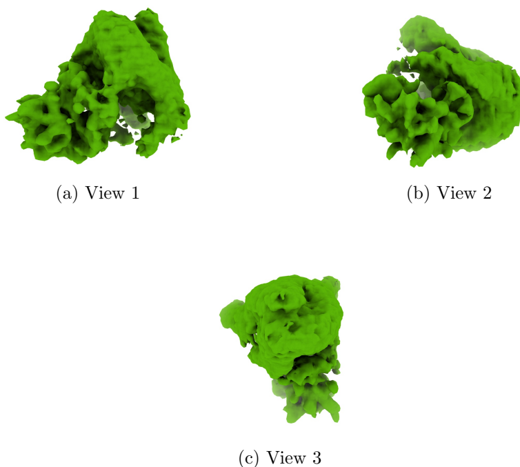
Figure 4: Isosurface at threshold=0.541000. Views generated by ChimeraX at a the following X, Y, Z angles: View 1 (0, -90, -90), View 2 (-90, 0, -90), View 3 (0, 0, 0).
