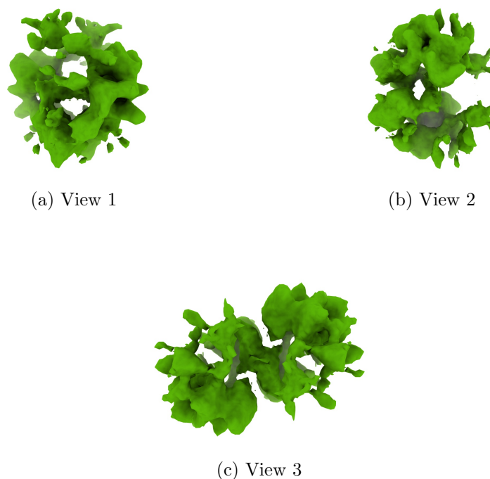
Figure 4: Isosurface at threshold=0.744000. Views generated by ChimeraX at a the following X, Y, Z angles: View 1 (0, -90, -90), View 2 (-90, 0, -90), View 3 (0, 0, 0).
