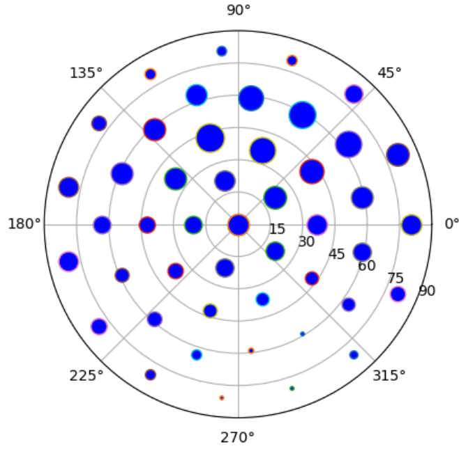
Figure 27: Histogram 2D of the best direction at each voxel. The azimuthal rotation is circular, while the tilt angle is the radius. The size of the point is proportional to the number of voxels whose maximum resolution is in that direction (this count can be seen in Fig. 26).
