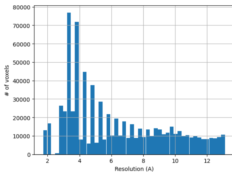
Figure 24: Histogram of the local resolution according to MonoRes.
