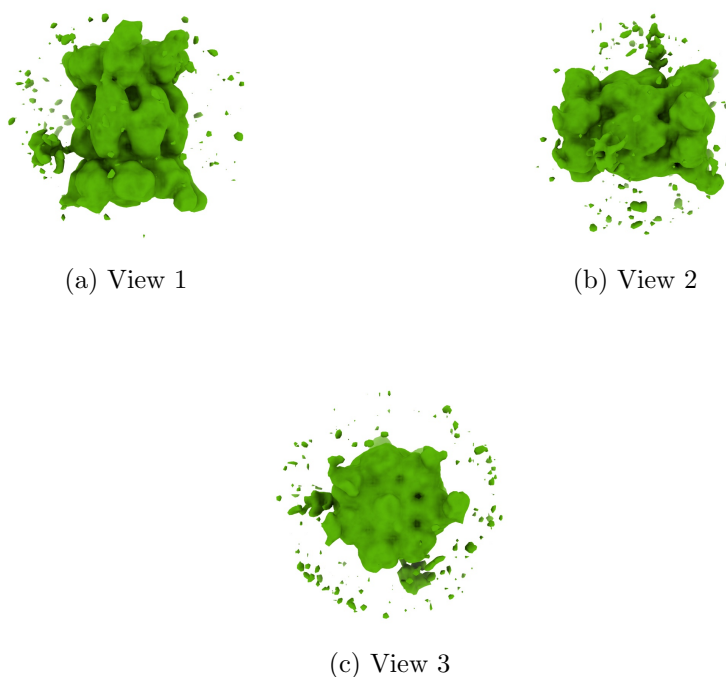
Figure 4: Isosurface at threshold=0.002200. Views generated by ChimeraX at a the following X, Y, Z angles: View 1 (0, -90, -90), View 2 (-90, 0, -90), View 3 (0, 0, 0).
